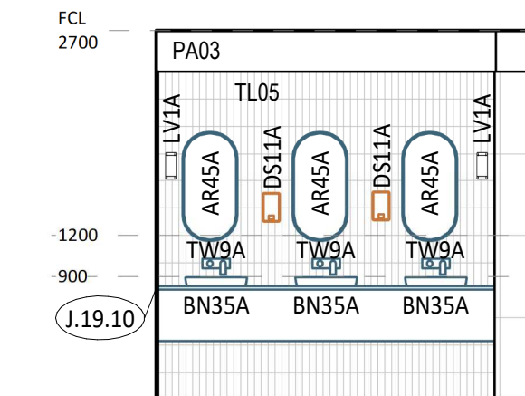
14 ELEVATION DETAIL 1 : 50
