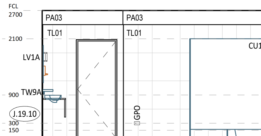
15 ELEVATION DETAIL 1 : 50
