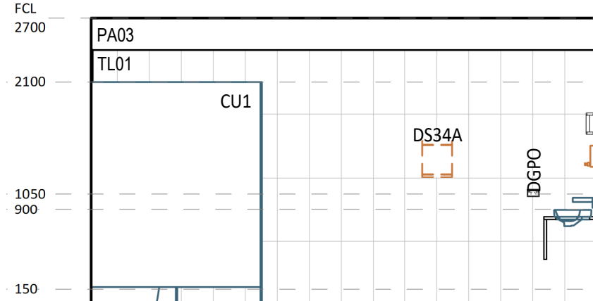
13 ELEVATION DETAIL 1 : 50
