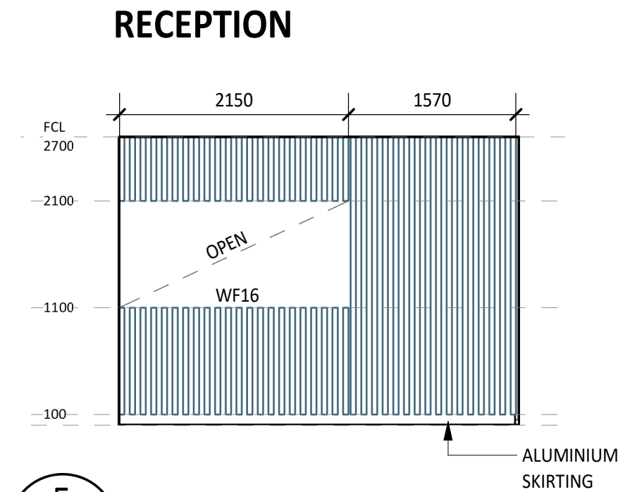
5 ELEVATION DETAIL 60-01 1:50
