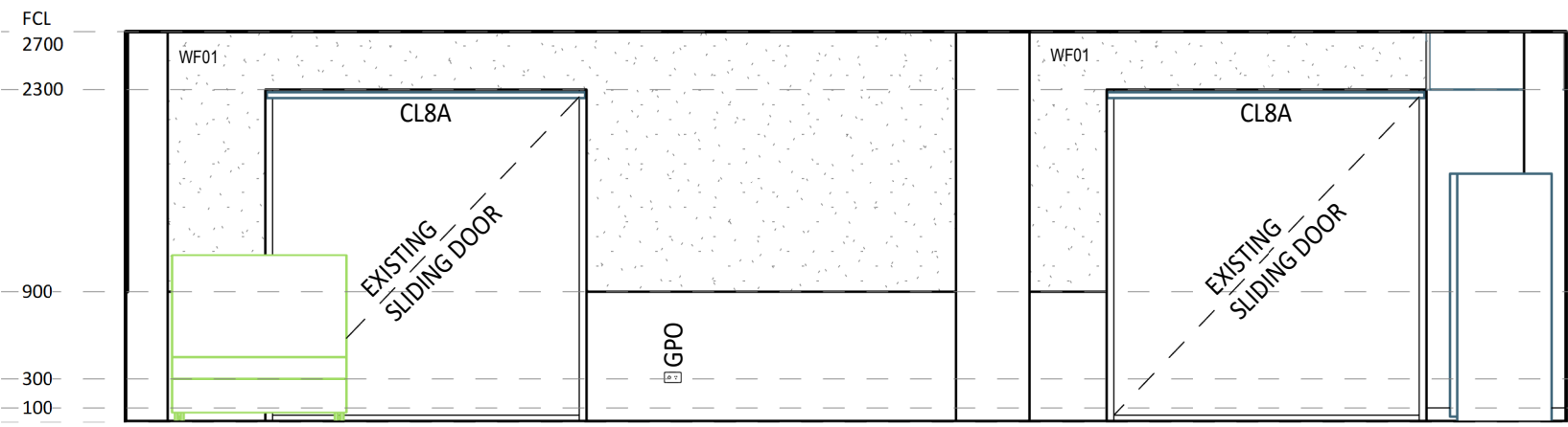
3 ELEVATION DETAIL 1 : 50
