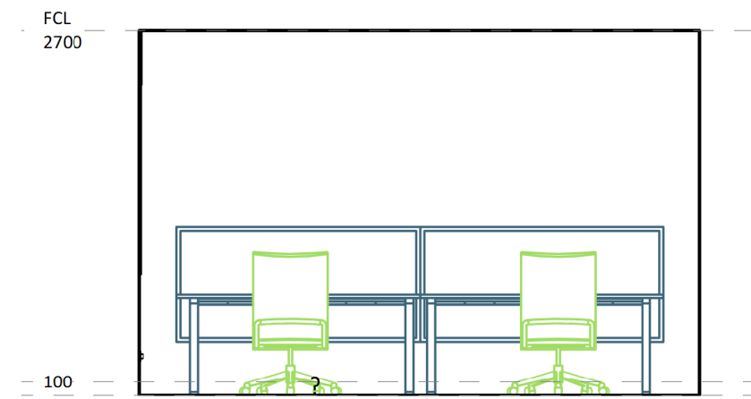
8 ELEVATION DETAIL 60-03 1 : 50
