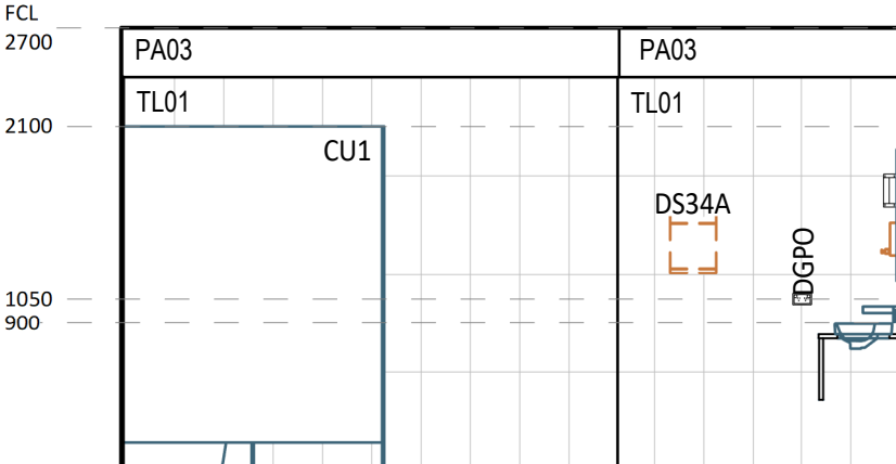
8 ELEVATION DETAIL 1 : 50
