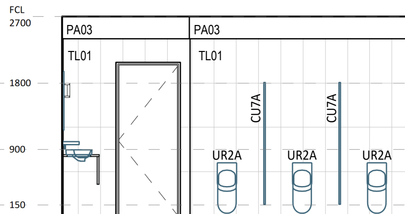
10 ELEVATION DETAIL 1 : 50
