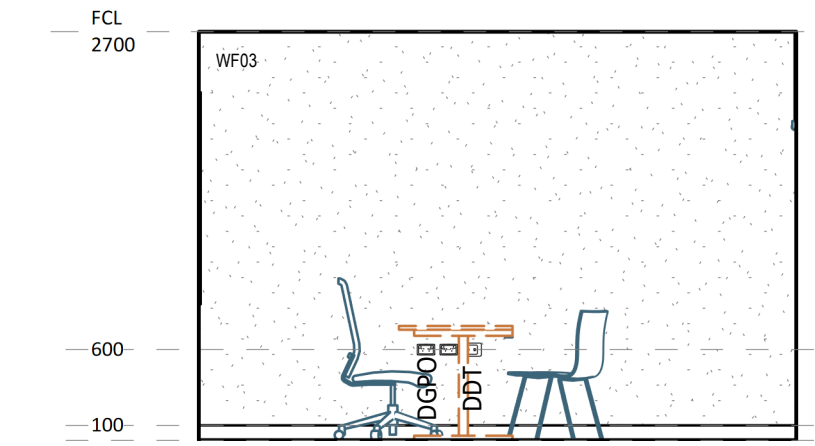
4 ELEVATION DETAIL 1 : 50
