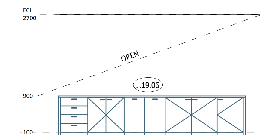
5 ELEVATION DETAIL 1 : 50
