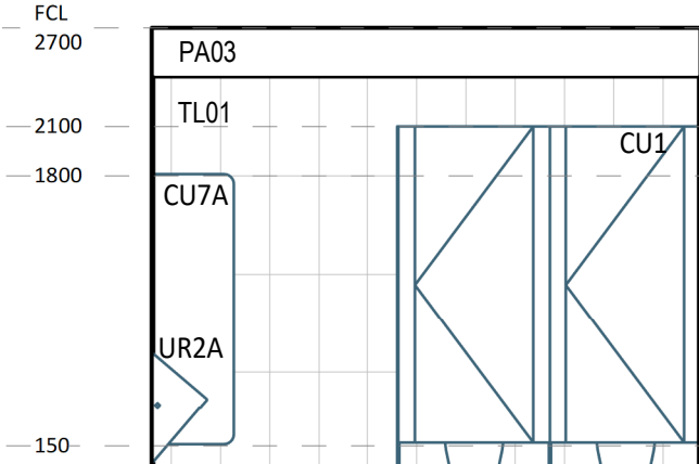
7 ELEVATION DETAIL 1 : 50
