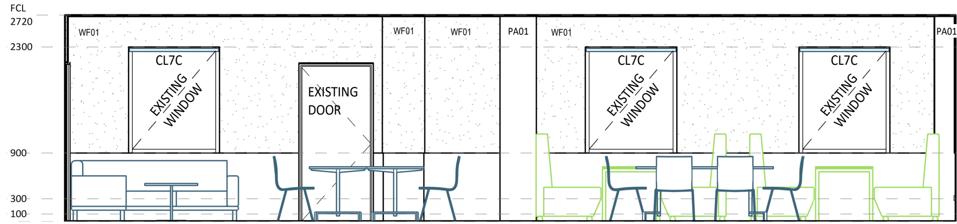
2 ELEVATION DETAIL 1 : 50
