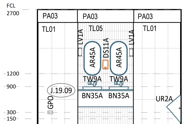
9 ELEVATION DETAIL 1 : 50
