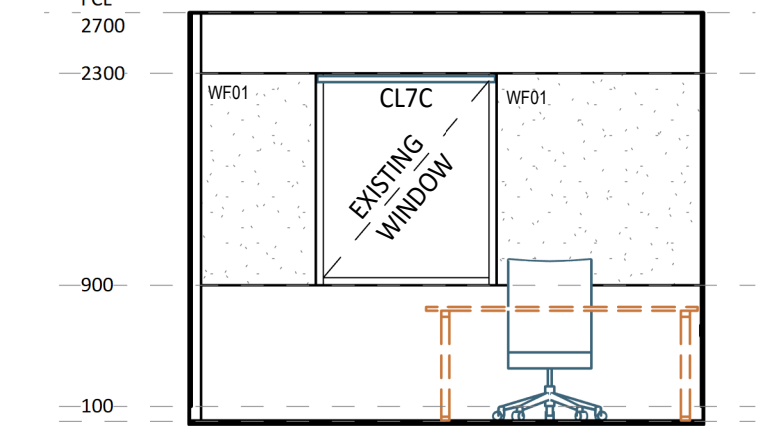
3 ELEVATION DETAIL 1 : 50
