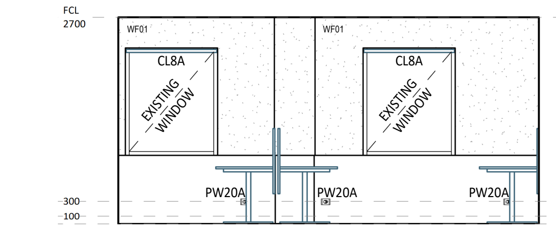
7 ELEVATION DETAIL 60-03 1 : 50
