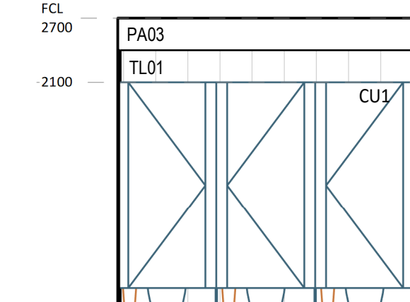
12 ELEVATION DETAIL 1 : 50
