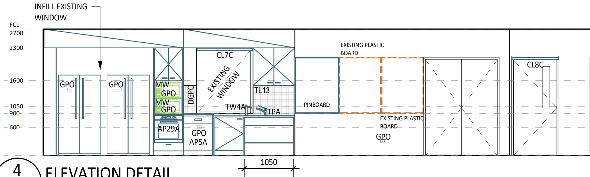
4 ELEVATION DETAIL 1 : 50
