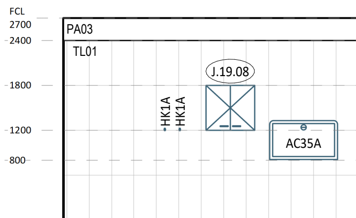
3 ELEVATION DETAIL 1 : 50
